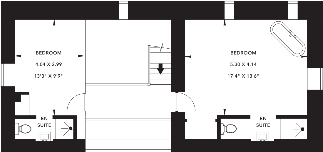
STONE BARN - FIRST FLOOR
